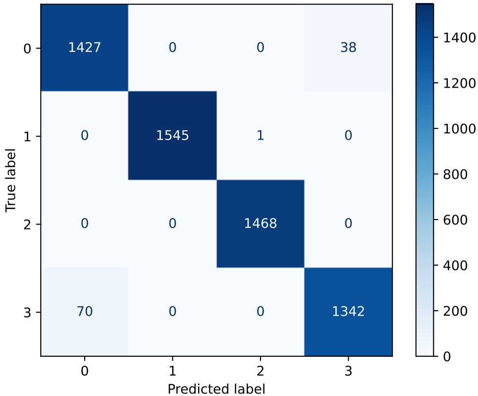
Fold 5 - Confusion Matrix
